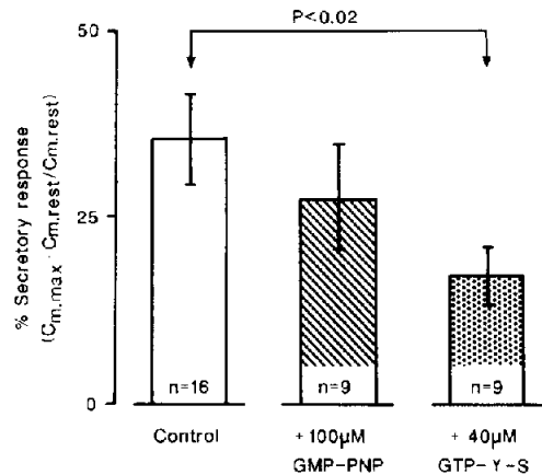
Fig.2. Suppressive effect of GTP analogues on the Ca-dependent secretory response. C_{m,max} , maximal C_m recorded; C_{m,rest} , initial resting C_m . Note the decrease in the secretory response in the added presence of GMP-PNP and GTP- \gamma -S in the pipette solution containing \sim 1 \mu M free Ca, when compared to the response in the presence of \sim 1 \mu M free Ca alone (control). Statistical test: The Welch's test for Behren's Fisher problem [29].
